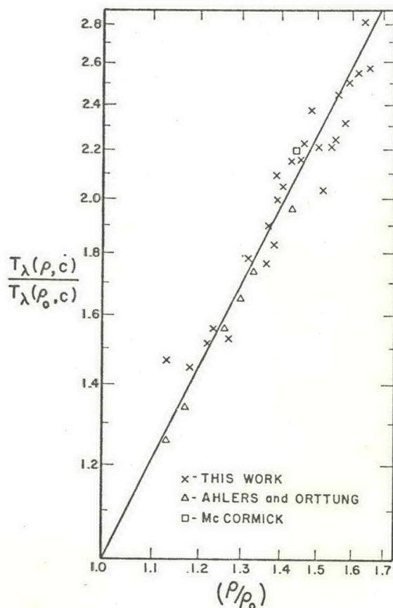
FIG. 8. Plot of the ratio of T_\lambda(\rho, c)/T_\lambda(\rho_0, c) versus relative density. The solid line has a slope of 2.0. The points from specific-heat measurements are deduced from Fig. 8 of Ref. 14.
